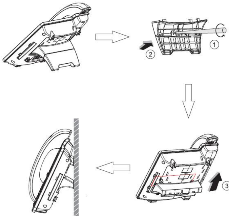
Figure 2 - Wall-mount Installation
